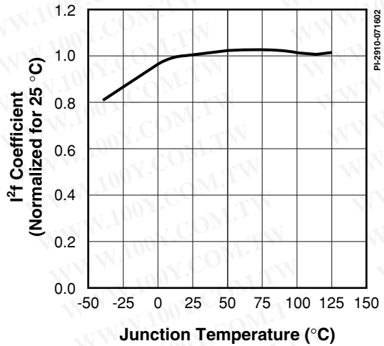
Figure 20. I 2 f Coefficient vs. Temperature.
